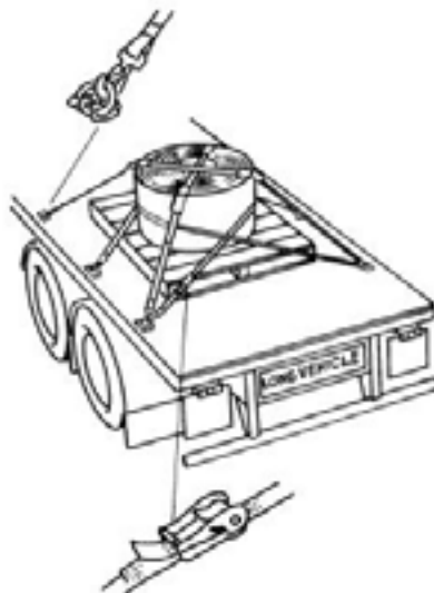
Example of securing of goods to a semi-trailer
